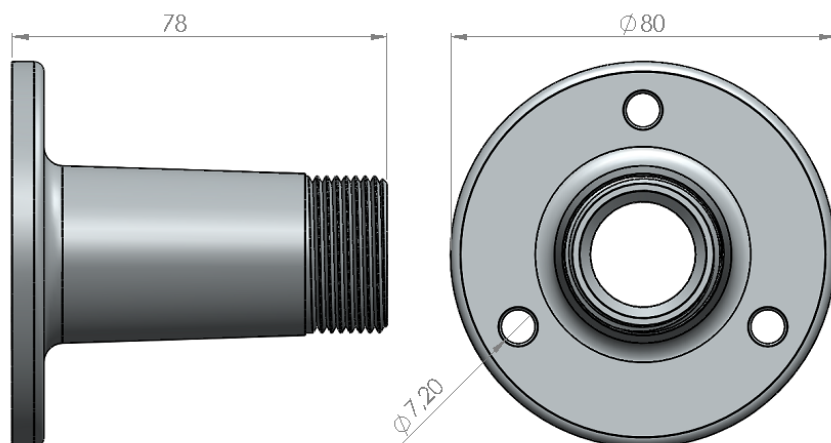
Outline Drawing
